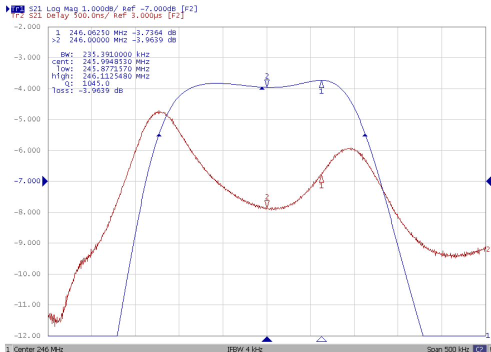
Fig2. Horizontal: 0.05MHz/Div Vertical: 1dB/Div
