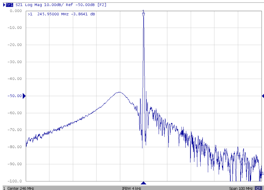
Fig4. Horizontal: 100MHz/Div Vertical: 10dB/Div
